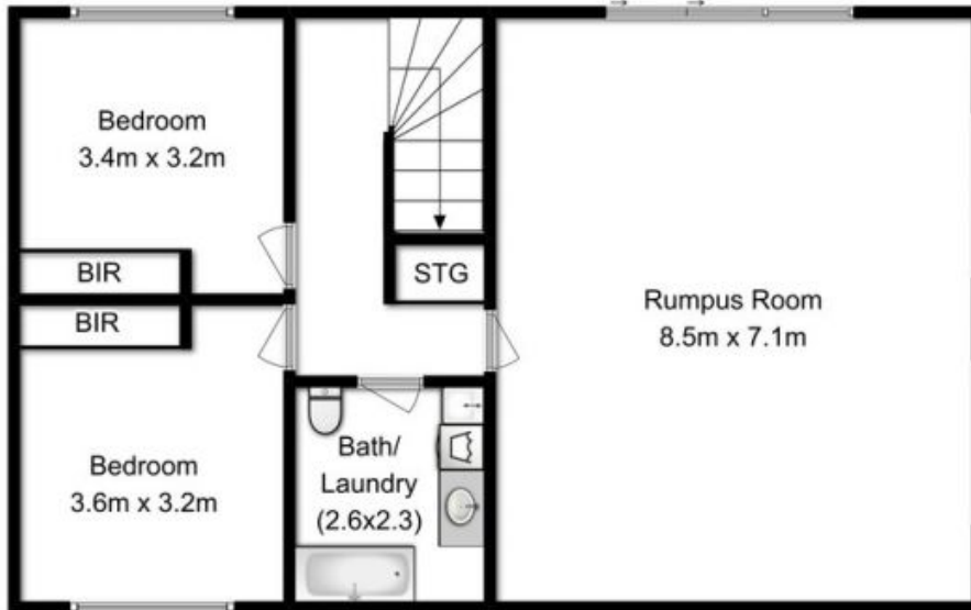
Ground Floor Approx Floor Area 83.8 Sqm
