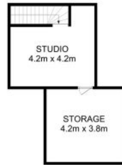
UPPER FLOOR
